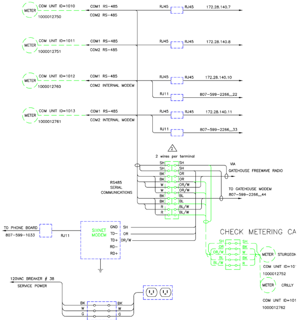
CABINET WIRING
