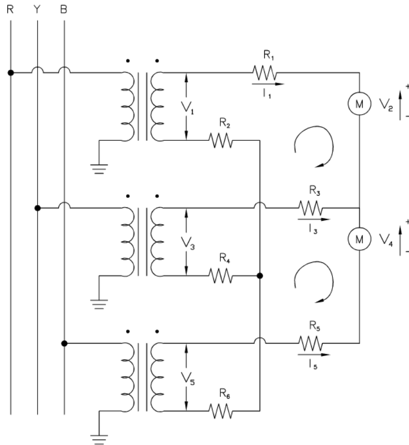
2 ELEMENT METERING USING 3 VTS
