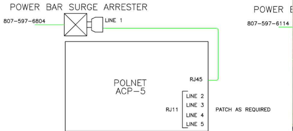
COM CABINET WIRING
